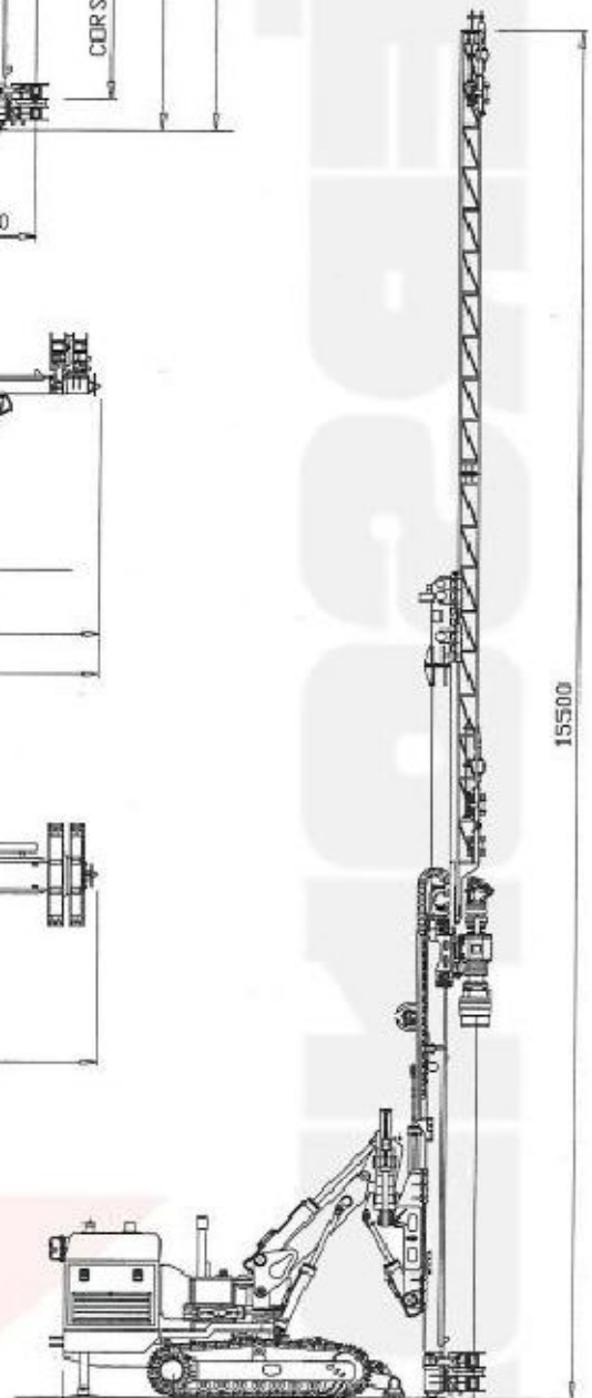
1250 2000 3250 1430 JET GROUTING CONFIGURATION
